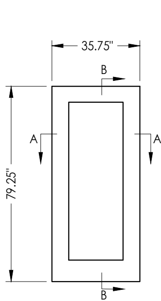
FIBERGLASS DOOR PANEL Plastpro 6' 8"
